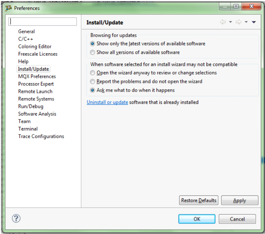
Figure 10. Uninstallation dialog
