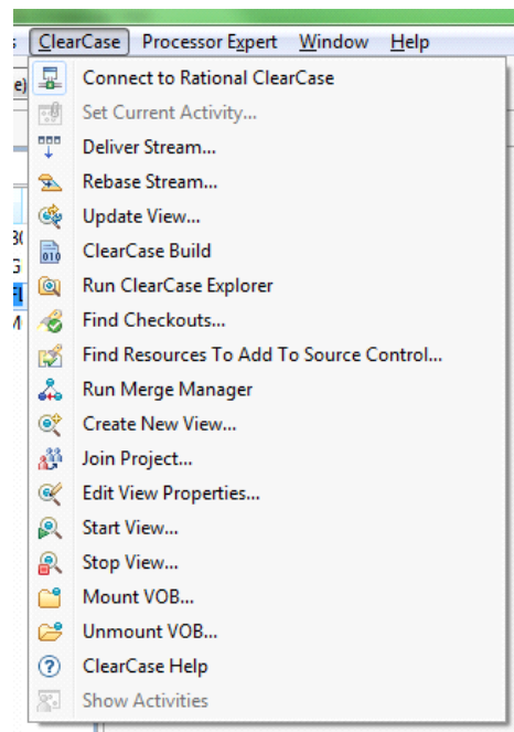
Figure 6. ClearCase menu
