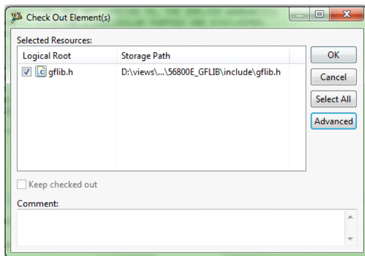
Figure 7. Check out
