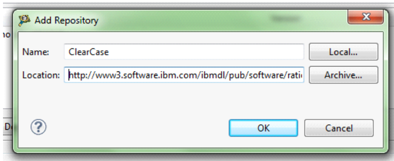
Figure 3. Plugin location
