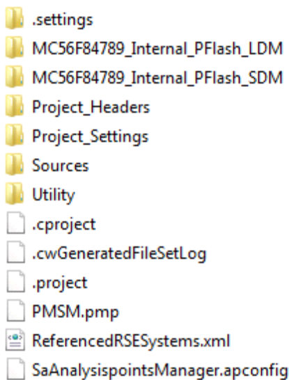
Figure 1. Project folder
