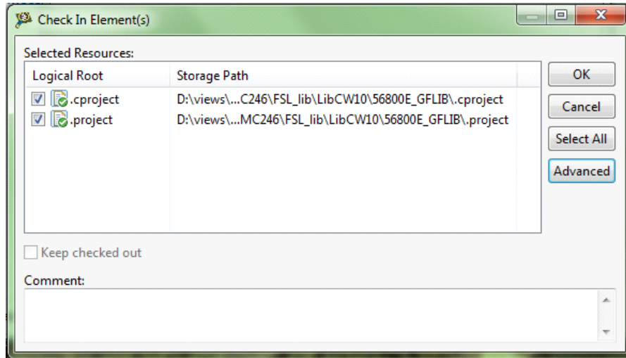
Figure 8. Project closing
