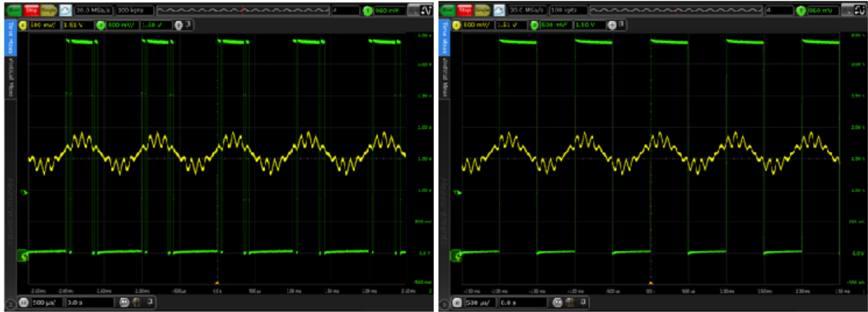
Figure 8. Input signal captured without and with hysteresis
