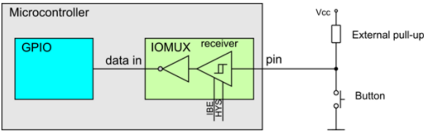
Figure 7. Connecting a button to an MCU
