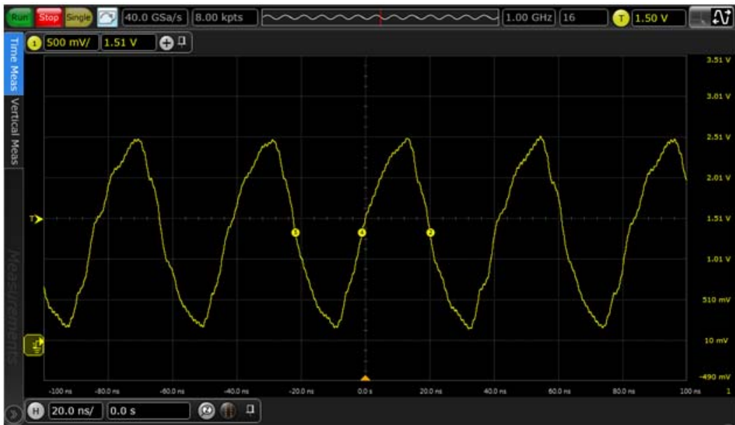
Figure 15. Incorrectly set DSE for a 24 Hz signal (DSE = 150 \Omega SRE = low, SPEED = 50 MHz)
