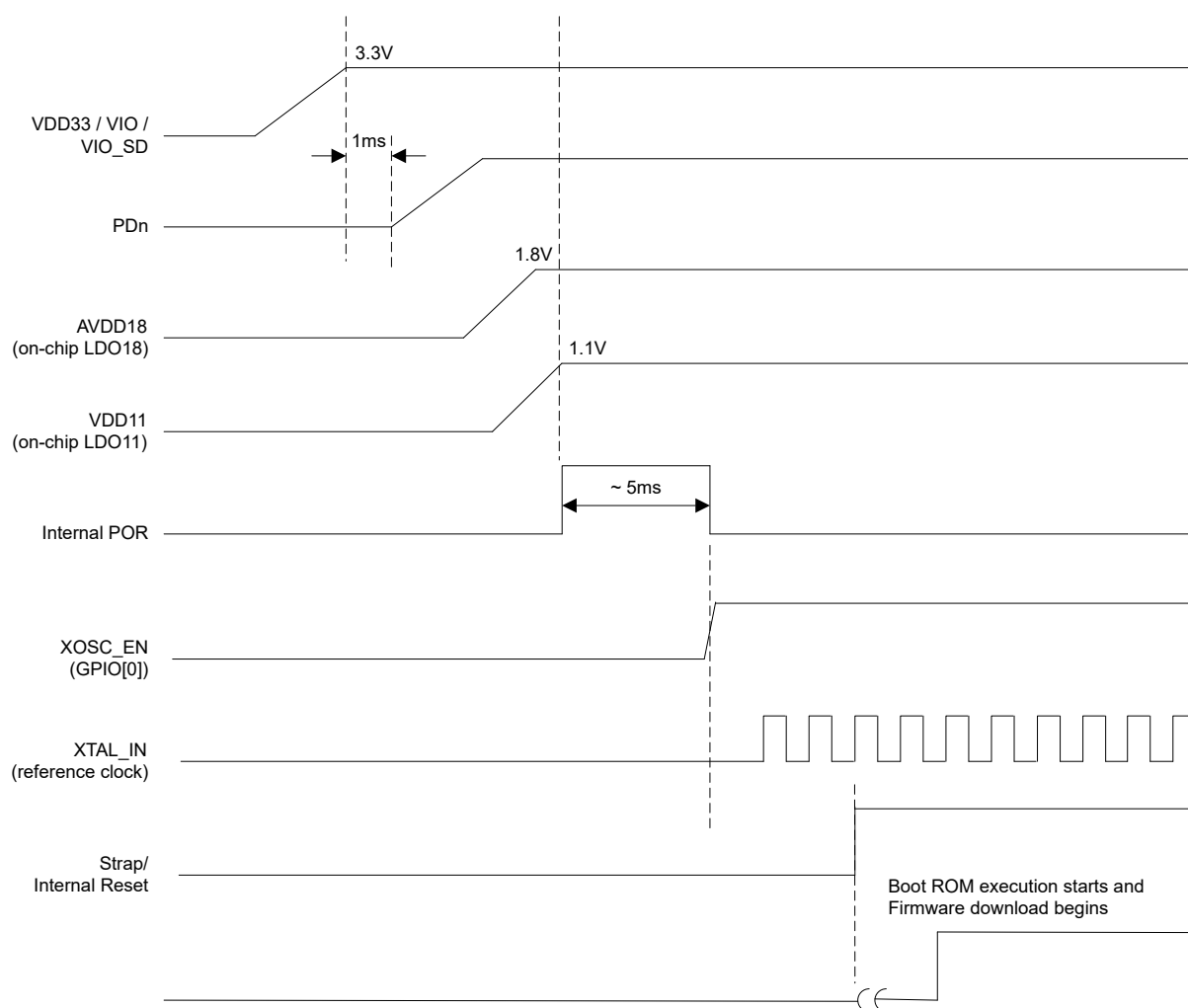
Figure 7. Power-up sequence for case 1 and PDn driven by host
