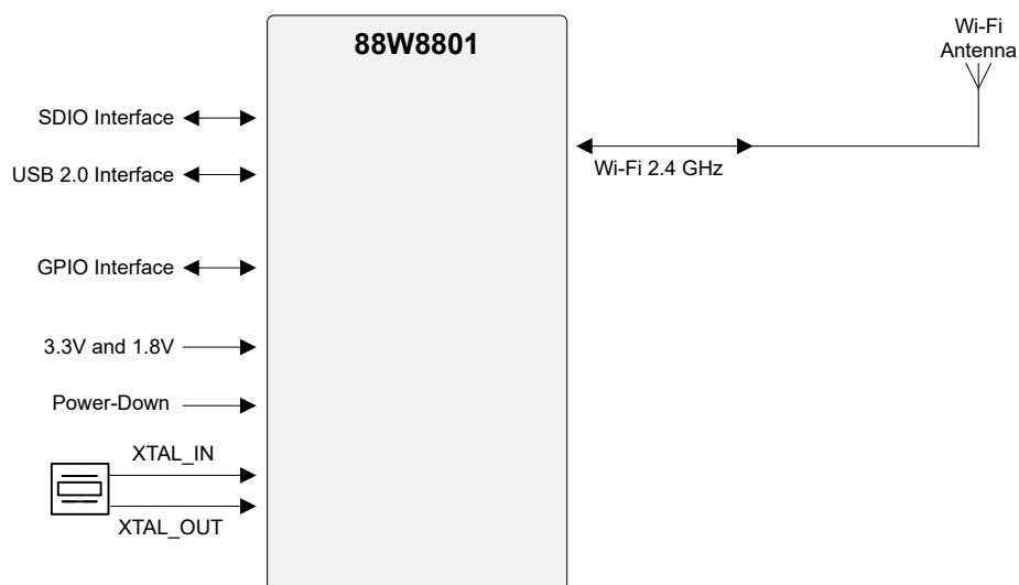
Figure 1. Application block diagram
