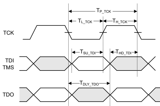
Figure 15. JTAG timing diagram
