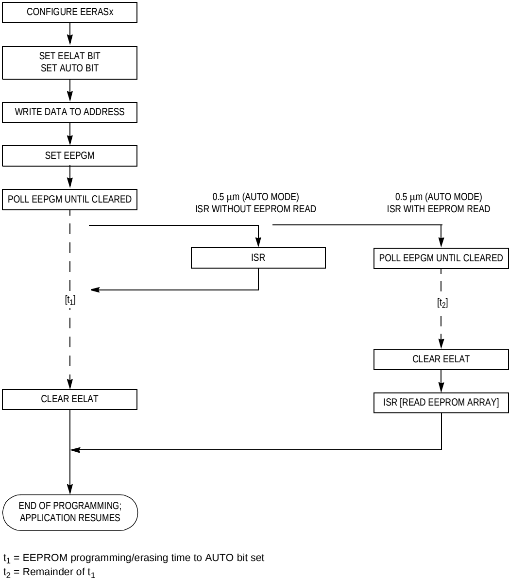
Figure 3. Program/Erase Flow — 0.5 μm (AUTO Mode)
