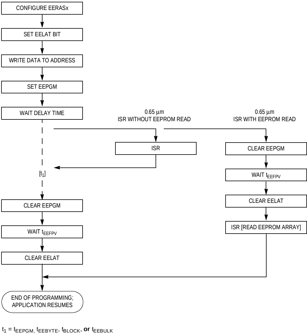
Figure 1. Program/Erase Flow — 0.65 μm
