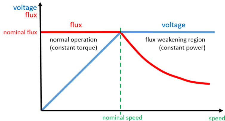
Figure 33. Flux weakening operating range
