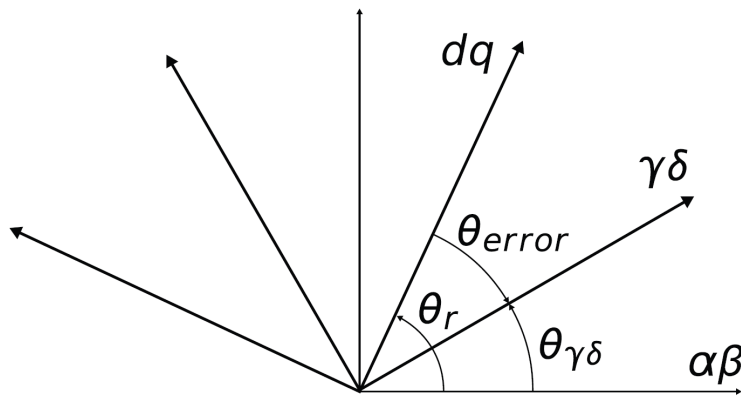
Figure 41. The estimated and real rotor dq synchronous reference frames
