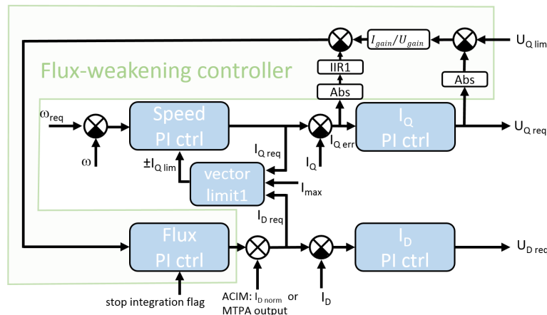
Figure 39. Flux weakening function in control block structure
