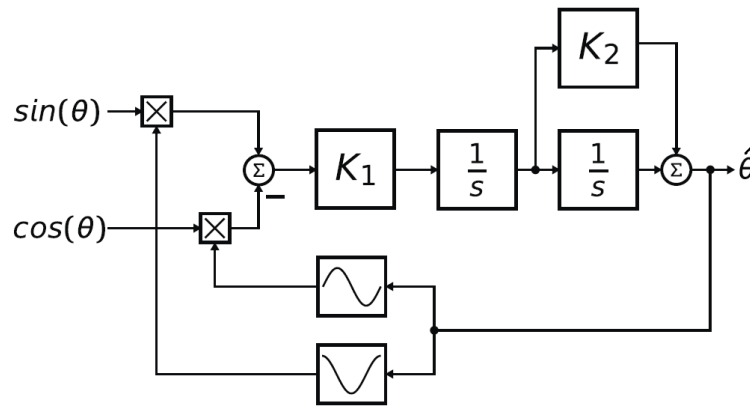
Figure 31. Block diagram of proposed PLL scheme for position estimation
