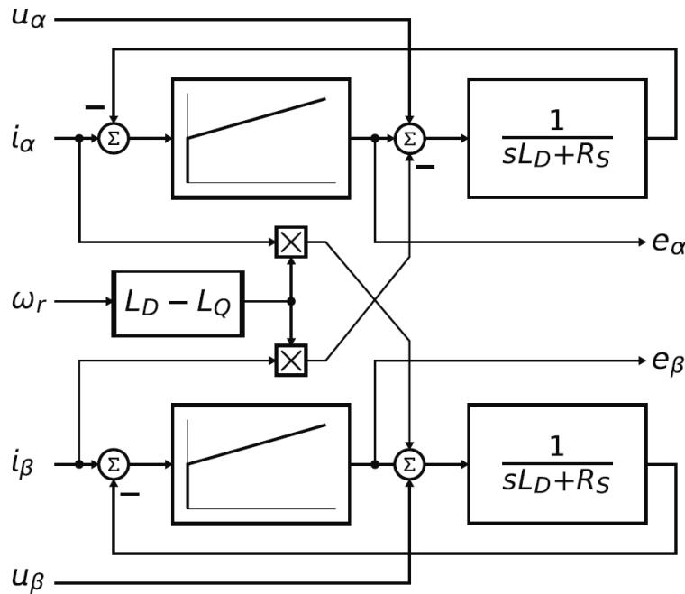
Figure 40. Block diagram of back-EMF observer
