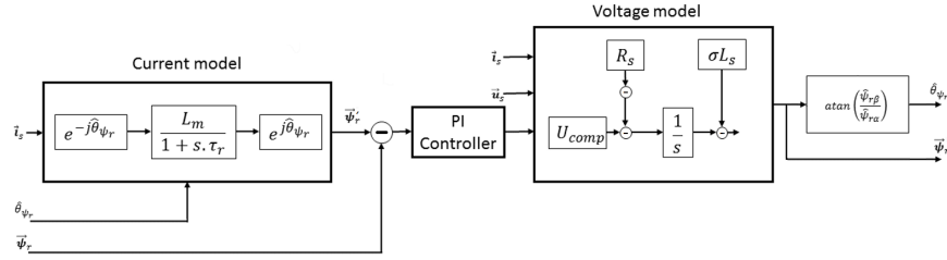
Figure 29. ACIM rotor flux observer block diagram
