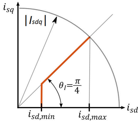
Figure 28. Minimal losses stator current vector trajectory with limits
