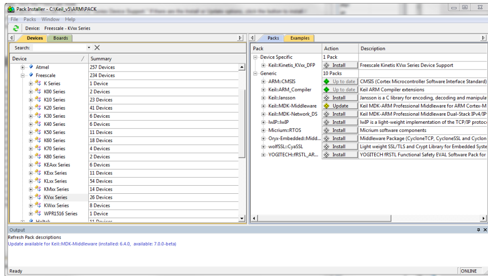
Figure 7. Pack Installer
