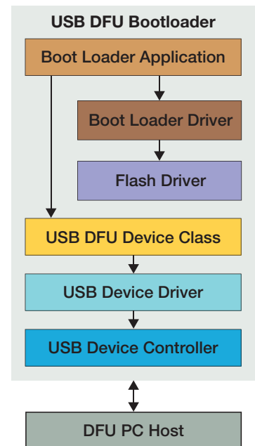
Figure 5. USB DFU bootloader architecture in the 12-axis sensor platform.
